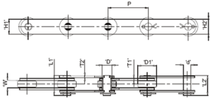
EUROPEAN SERIES (BS) - SOLID PIN CHAINS
