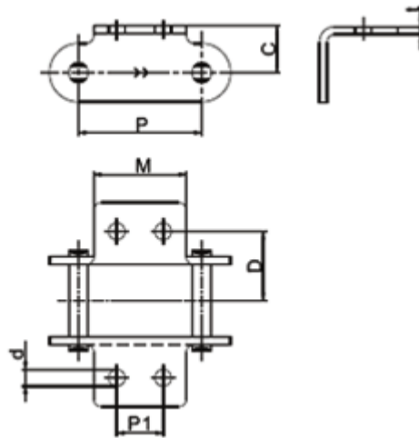
DOUBLE PITCH A2, K2 ATTACHMENTS
